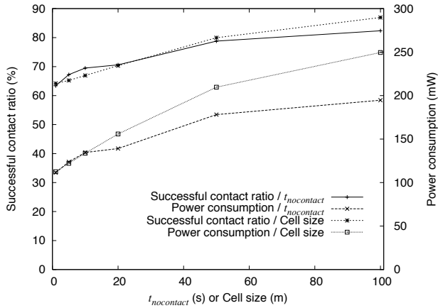
Fig. 10. Performance of the adaptive recent-activity scheme versus t_{nocontact} and performance of the adaptive location-based scheme versus cell size
