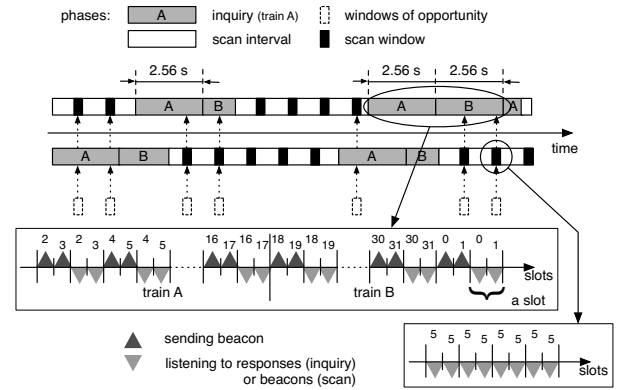
Fig. 1. Bluetooth discovery process
