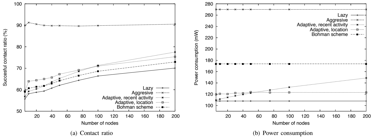
Fig. 8. Performance of the five schemes versus number of nodes
