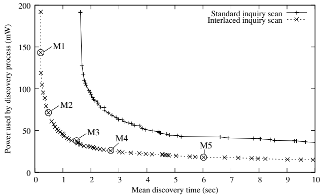
Fig. 4. Discovery time versus power consumption curve. M1 through M5 are discovery modes we use in the ad-hoc network simulation.
