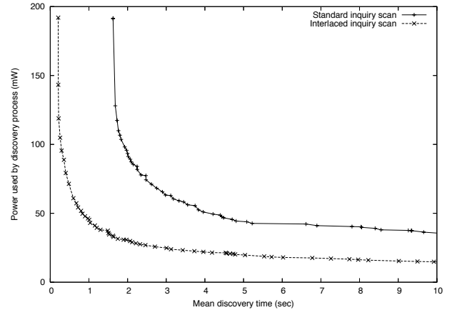
Fig. 3. Mean discovery time vs. power consumption of the discovery process
