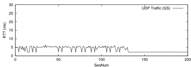
Figure 12: QoS control, RTT of EF class.
