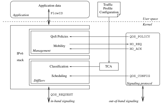
Figure 6: Protocol structure of a mobile host.
