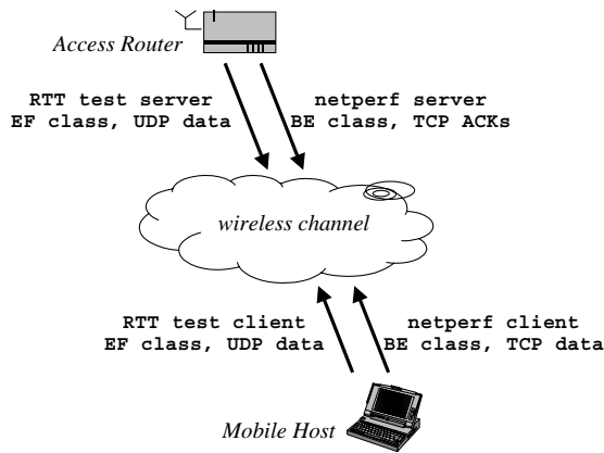
Figure 8: Experimentation set up.
