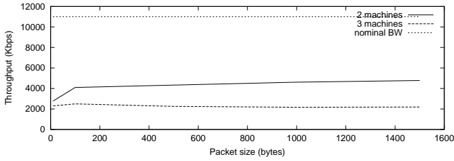
Figure 5: The useful bandwidth in the 802.11b wireless LAN.
