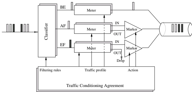
Figure 2: Edge router functions.
