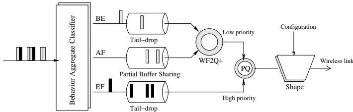
Figure 3: Core router functions.
