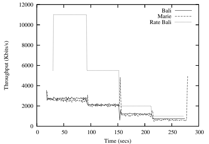
Fig. 6. Measured throughput in Mb/s for two hosts, UDP traffic
